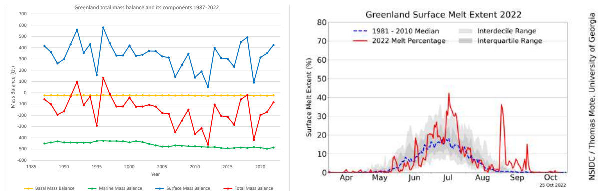
Figure 10: (left) Components of the total mass balance of the Greenland Ice Sheet 1987-2022. Blue: Surface mass balance (SMB), green: marine mass balance (MMB), orange: basal mass balance (BBM), red: total mass balance (TMB), the sum of SMB, MMB and BBM. Mankoff et al. (2021), updated and redrawn by M. Stendel. (right) Greenland Ice Sheet melt extent, 2022.. Image and analysis courtesy of Thomas Mote, U.S. National Snow and Ice Data Center.
